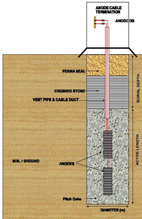
DISTRIBUTIVE, DEEP AND SHALLOW VERTICAL ANODE BED ARRANGEMENT
